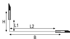
Alluminio - CPMP/AS H = L1 + 13 \text{ mm} B = L2 + 13 \text{ mm}
